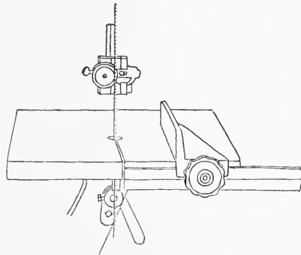
FIG. 184. RIPPING FENCE ON BAND-SAW.
